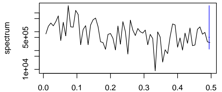
Remainder
