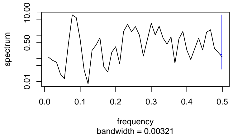
Standardized Residuals
