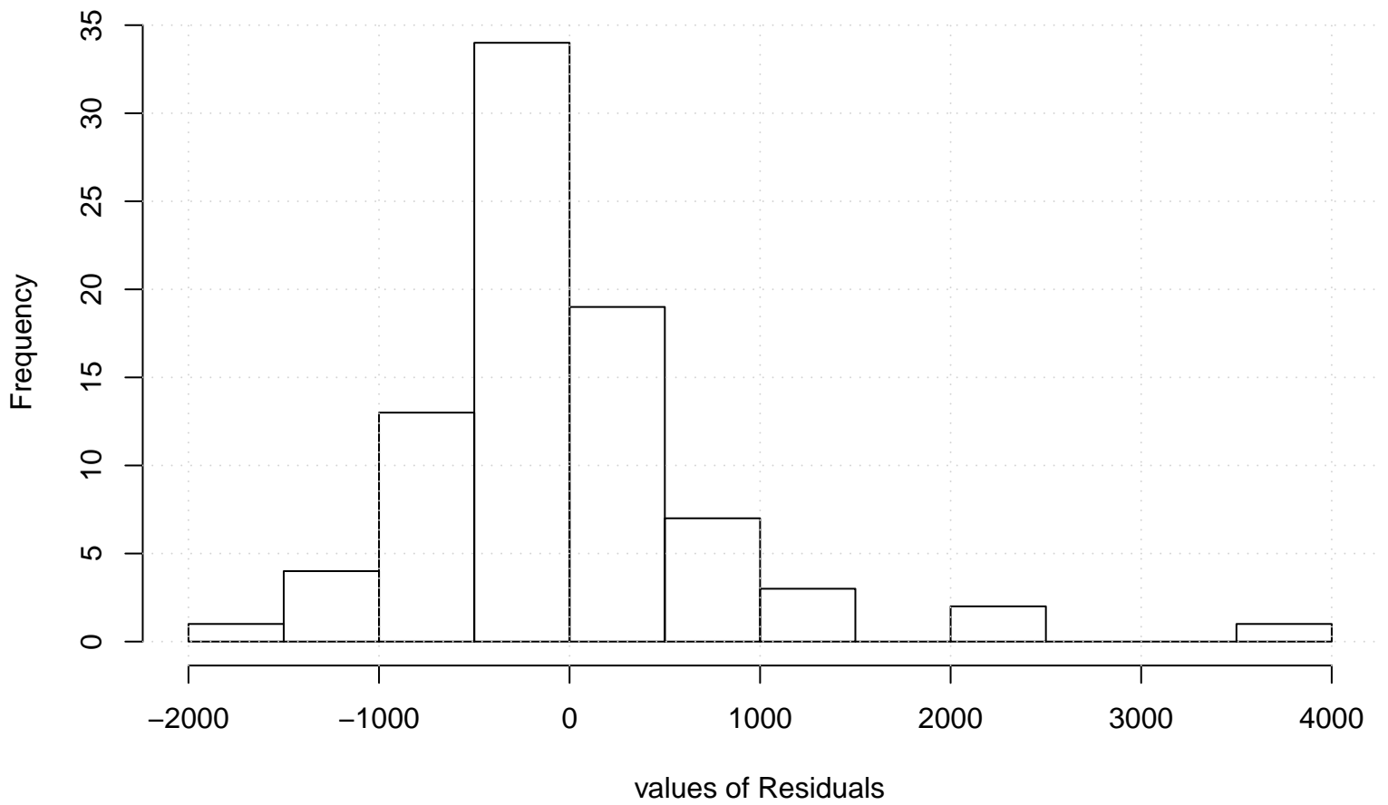
Residual Histogram
