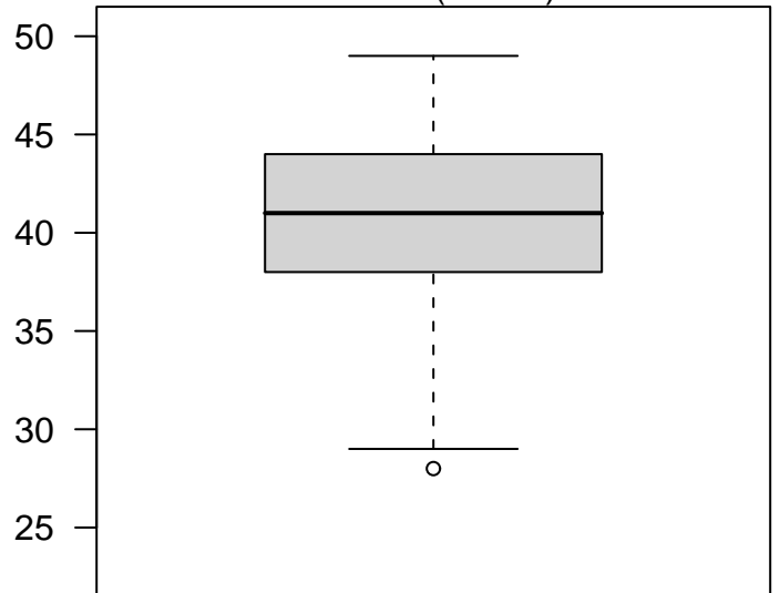
Node 3 (n = 91)
