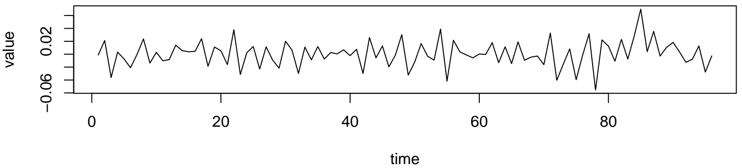
Working Time Series ( \lambda=-0.6 , d=1 , D=2 )
