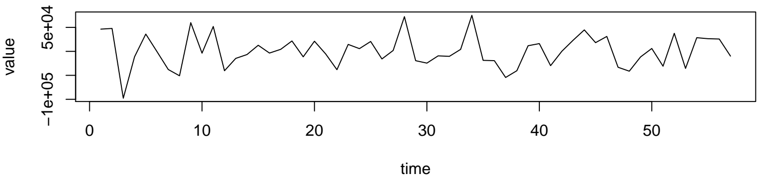
Working Time Series (lambda=1, d=2, D=0)
