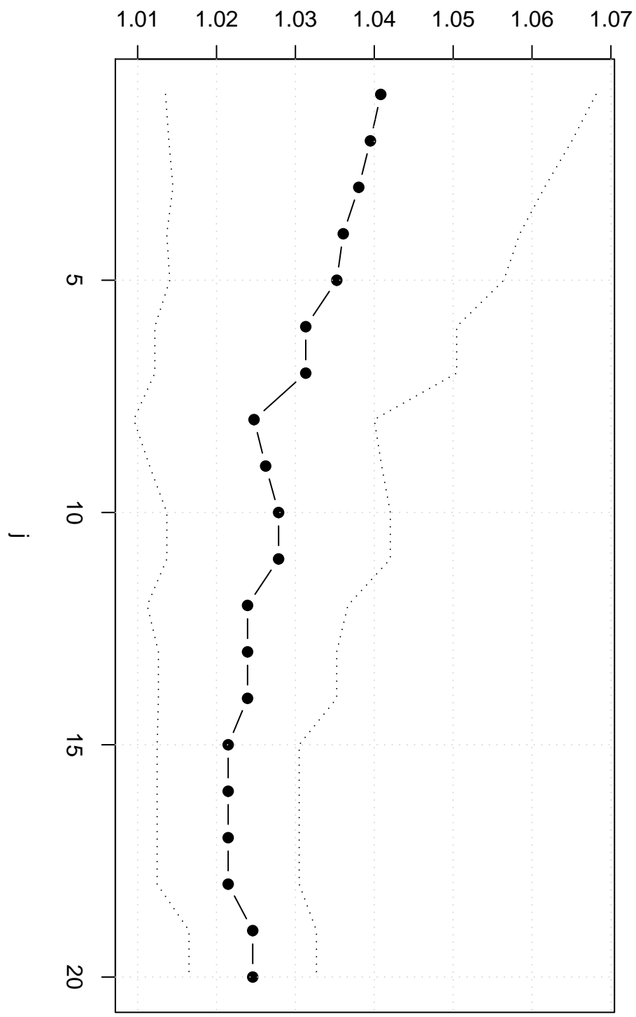
Winsorized Mean(j/n)
