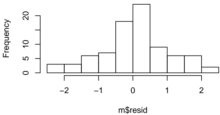
Residual Histogram
