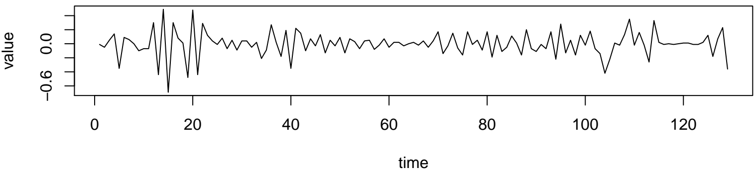
Working Time Series (lambda=1, d=2, D=0)
