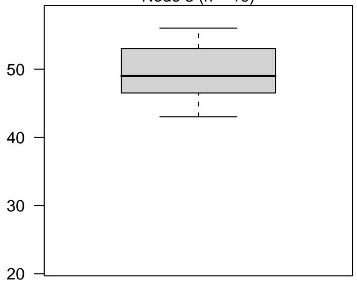
Node 3 (n = 19)
