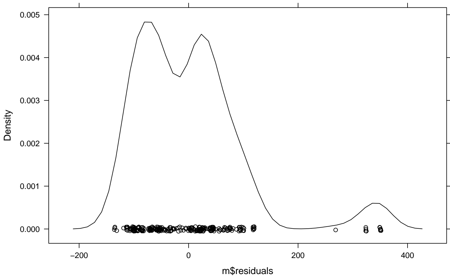
Density Plot
