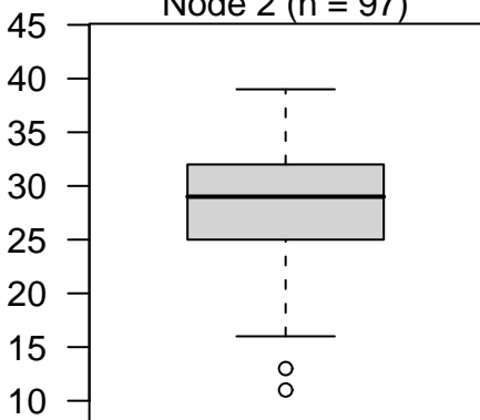
Node 2 (n = 97)
