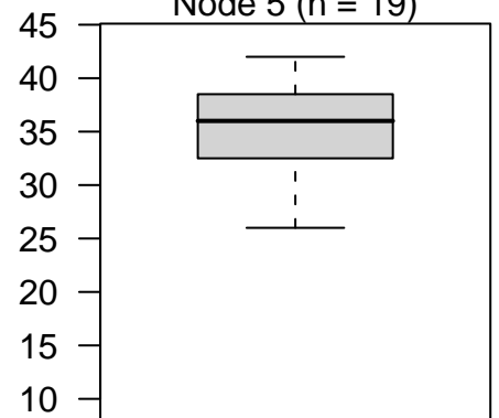
Node 5 (n = 19)
