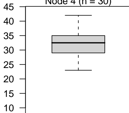
Node 4 (n = 30)
