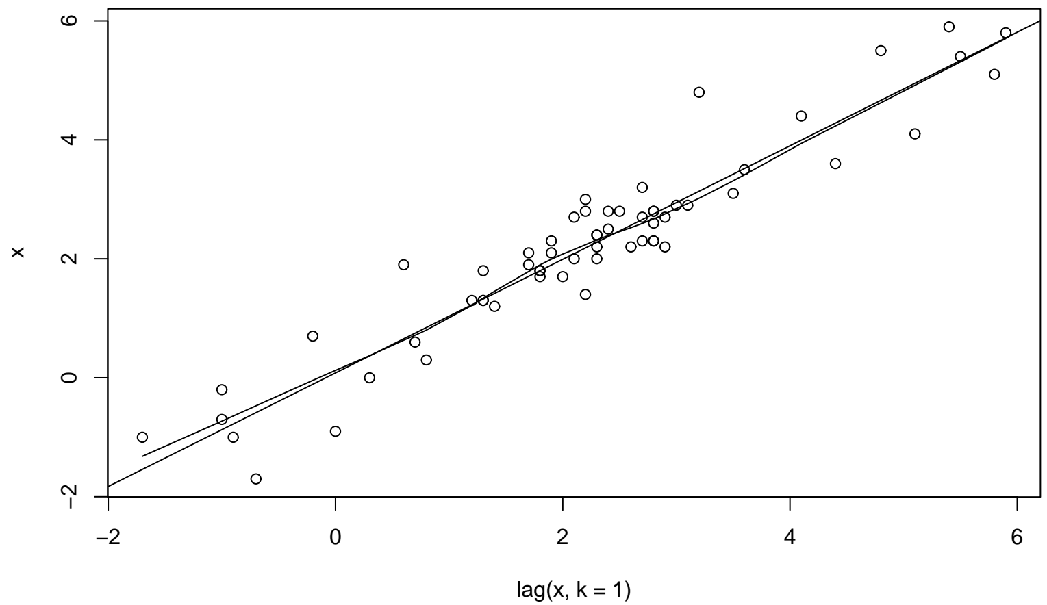
Lag plot (k=1), lowess, and regression line
