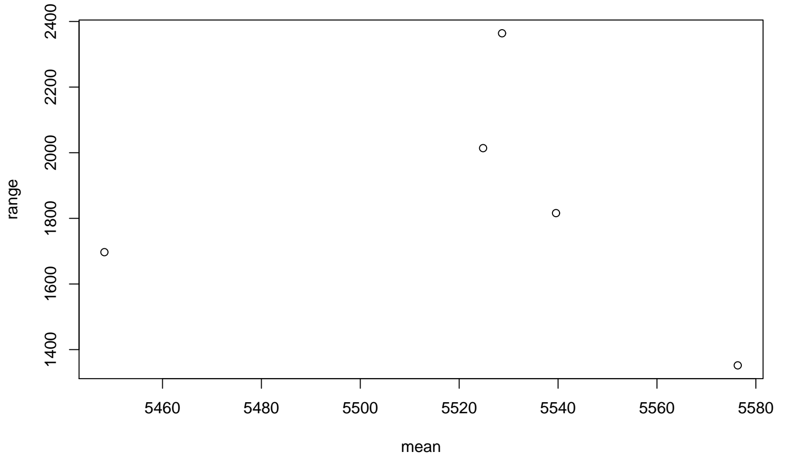
Range-Mean Plot
