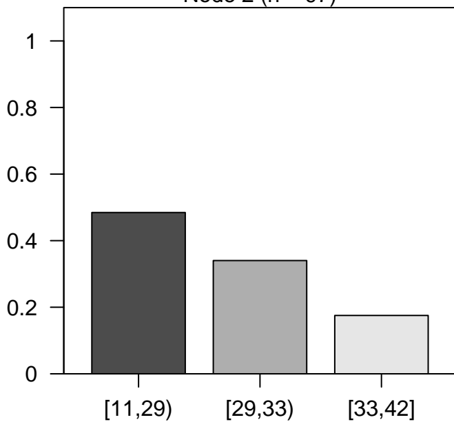
Node 2 (n = 97)
