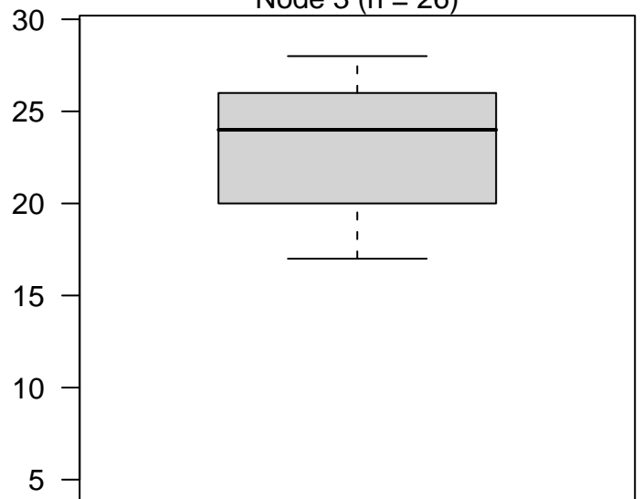
Node 3 (n = 26)
