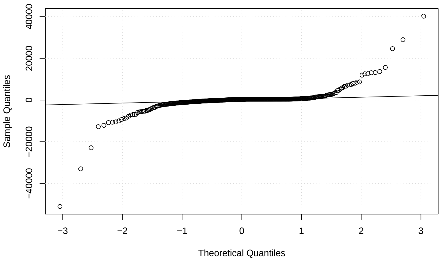
Residual Normal Q-Q Plot
