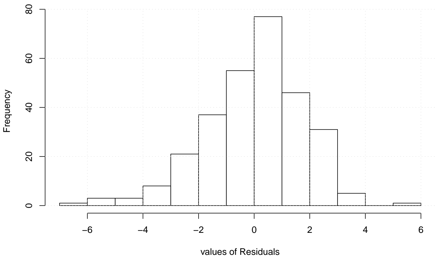
Residual Histogram
