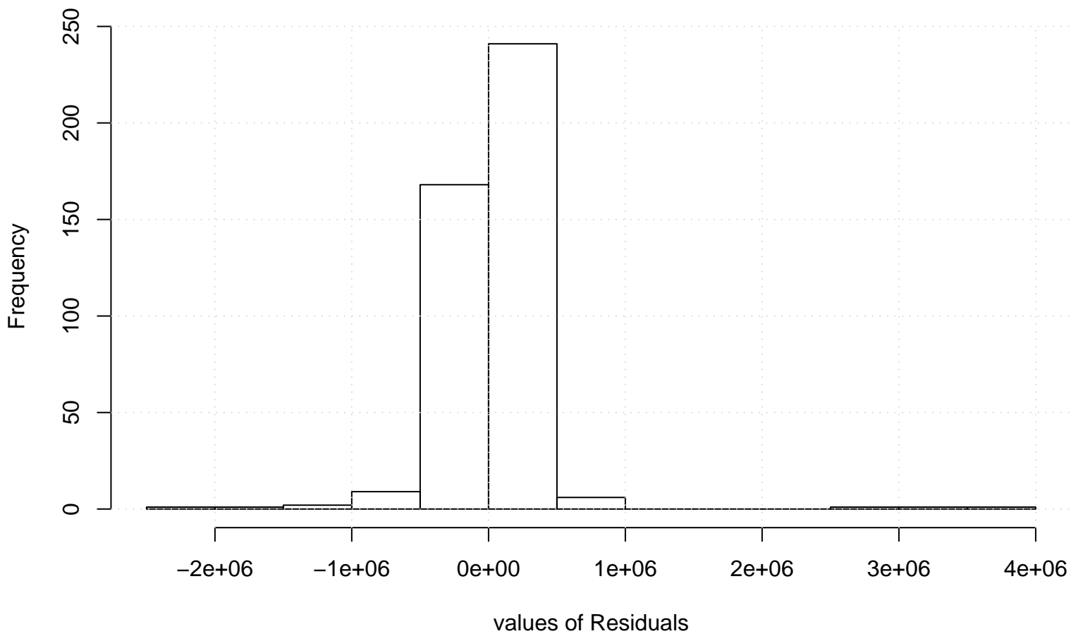
Residual Histogram
