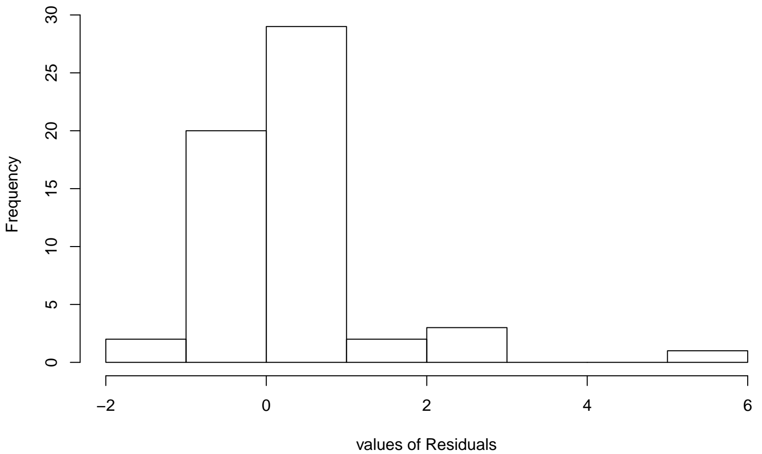
Residual Histogram
