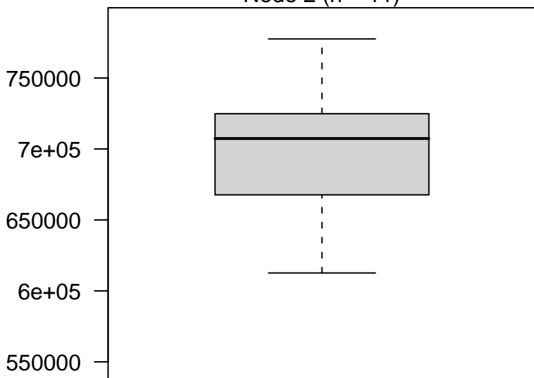
Node 2 (n = 11)
