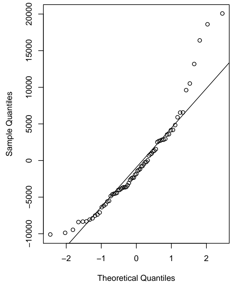
Residual Normal QQ Plot
