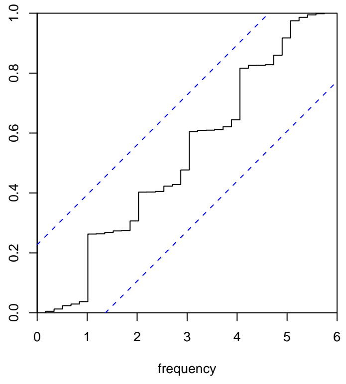
Residual Cumulative Periodogram
