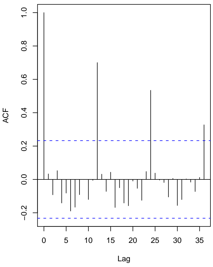
Residual ACF
