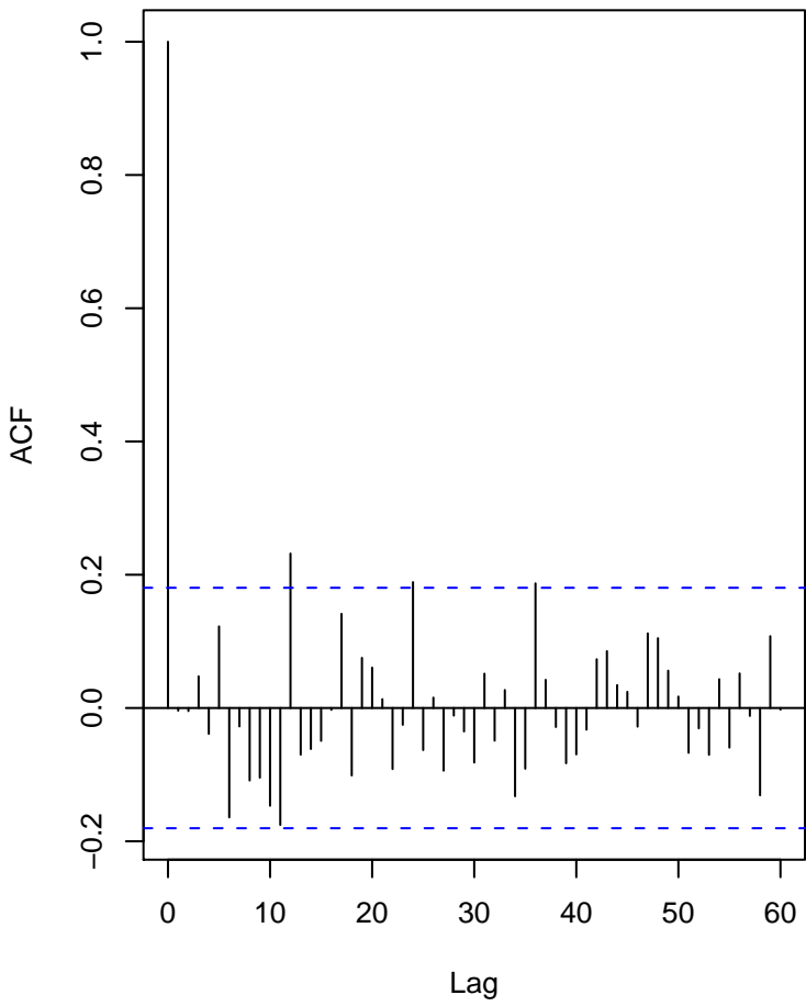
Residual ACF
