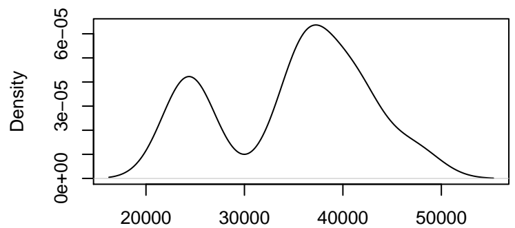
Kernel Density Plot of Predictions
