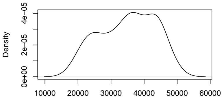
Kernel Density Plot of Actuals
