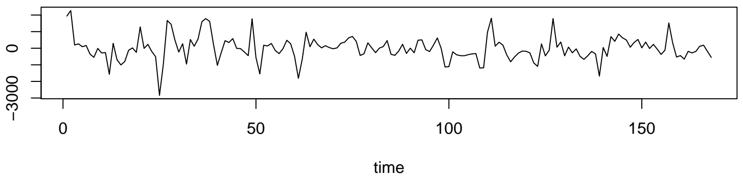
Working Time Series ( \lambda=1 , d=0 , D=1 )
