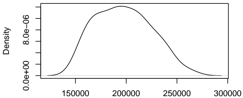
Kernel Density Plot of Actuals
