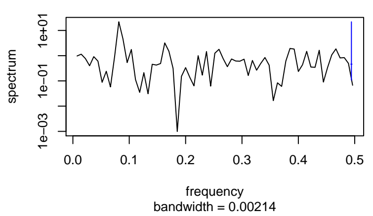
Standardized Residuals
