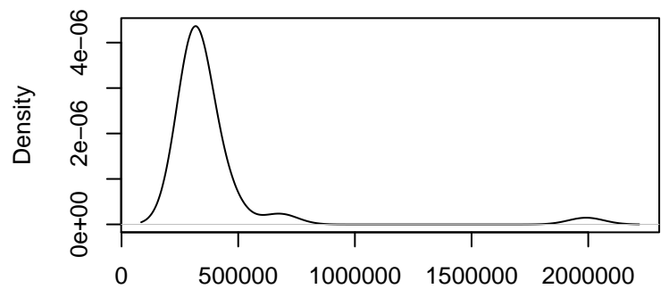
Kernel Density Plot of Predictions
