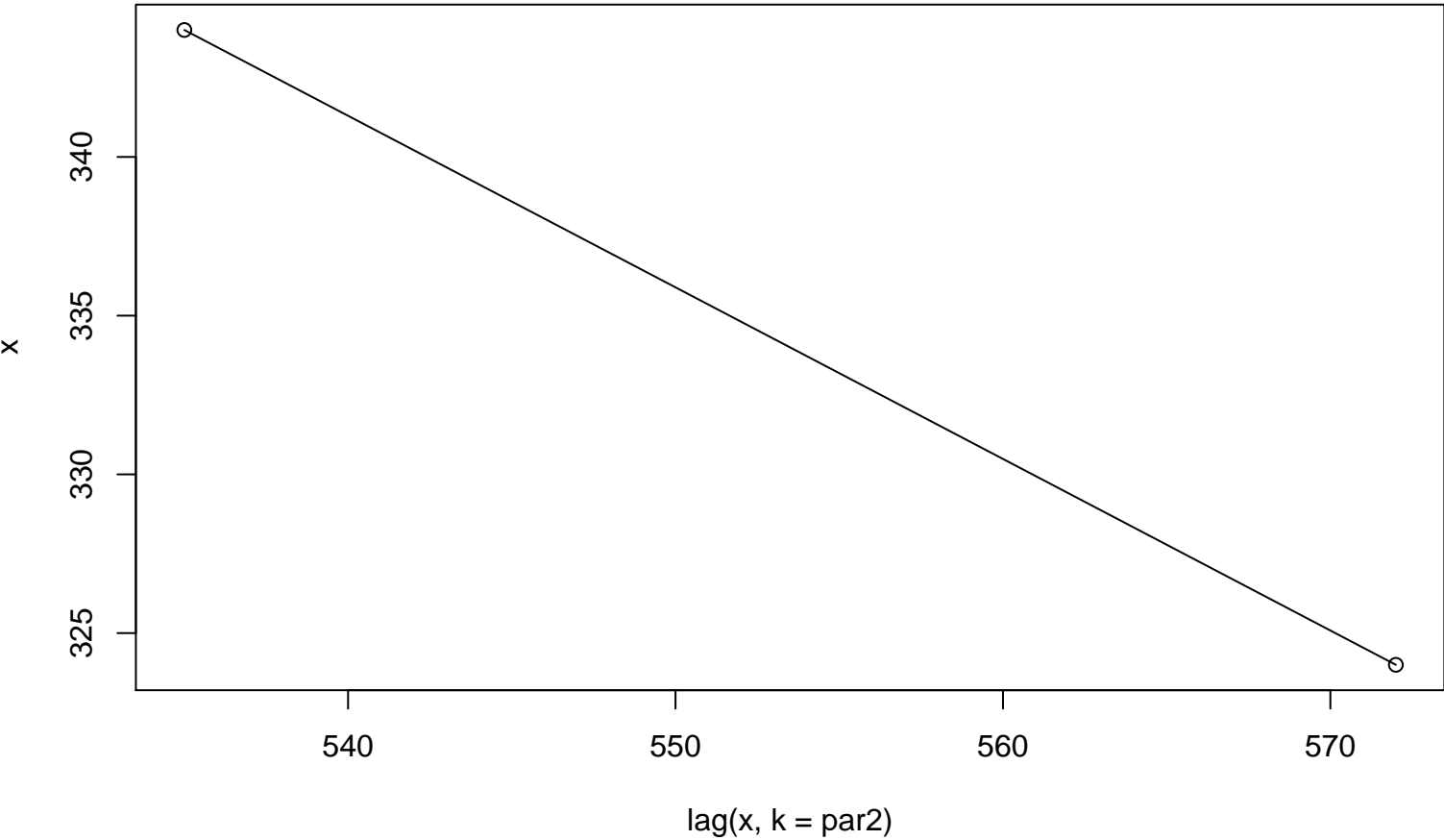
Lag plot (k=28), and lowess
