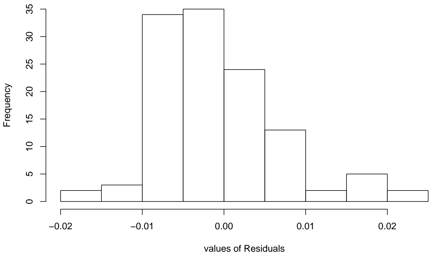
Residual Histogram
