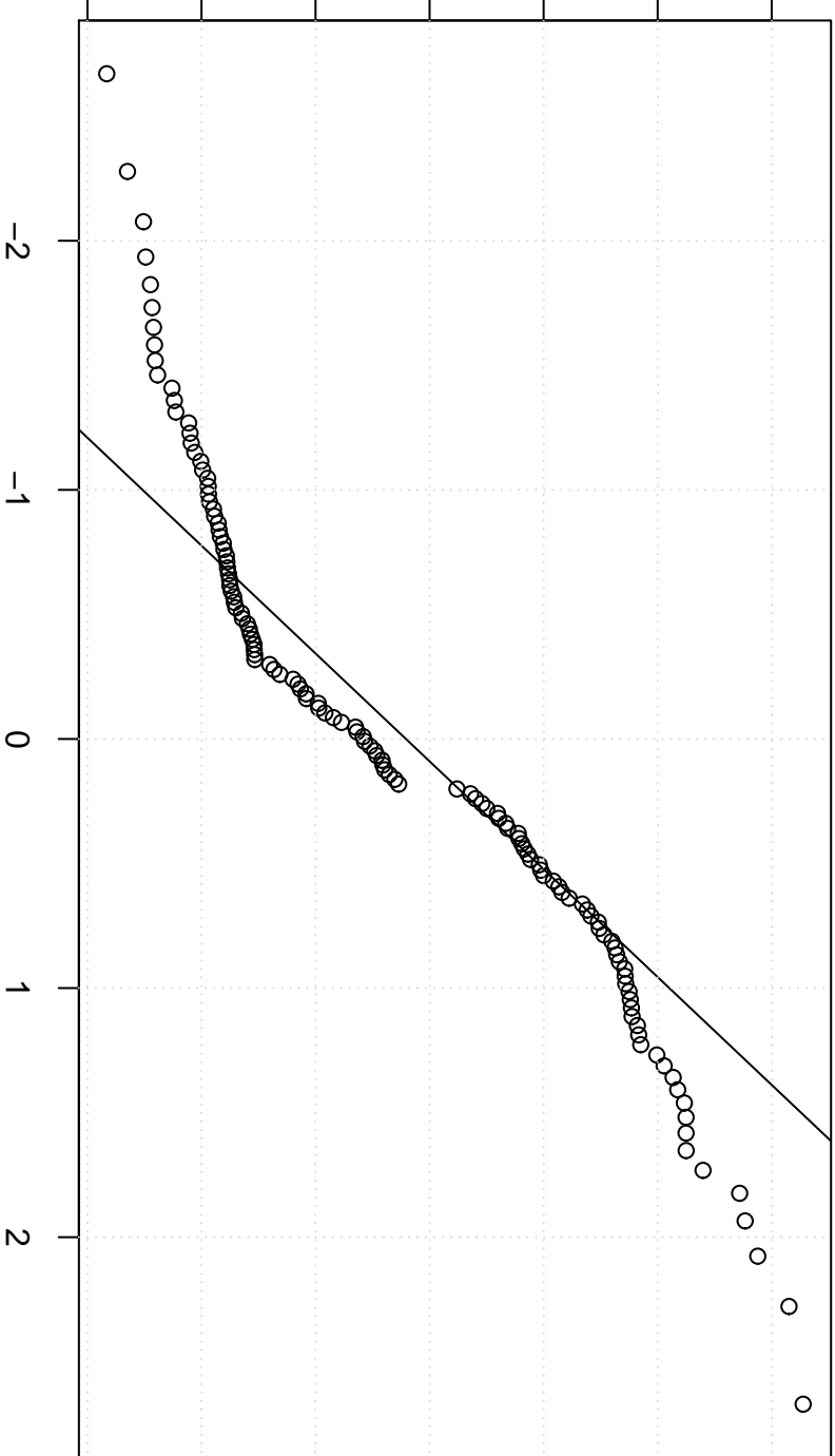
Theoretical Quantiles
