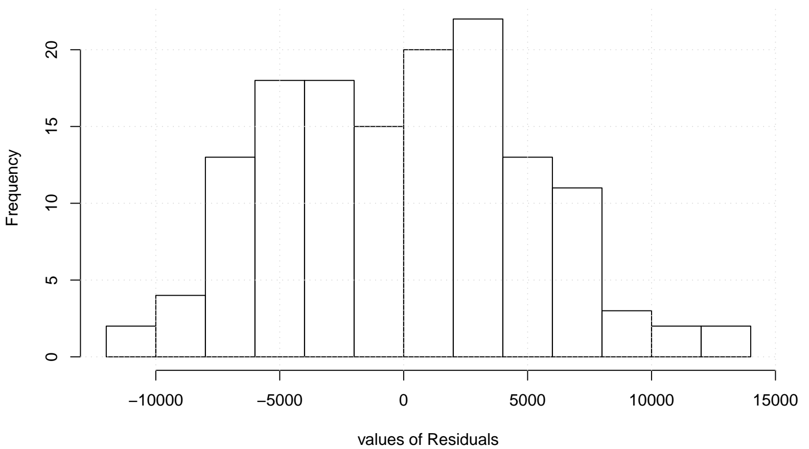
Residual Histogram
