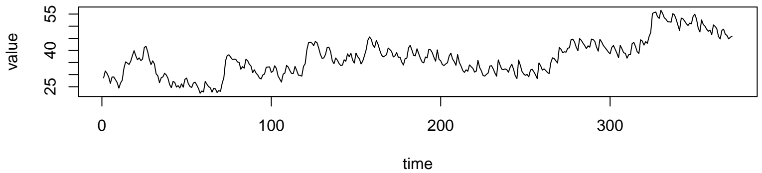
Working Time Series ( \lambda=0.5 , d=0 , D=0 )
