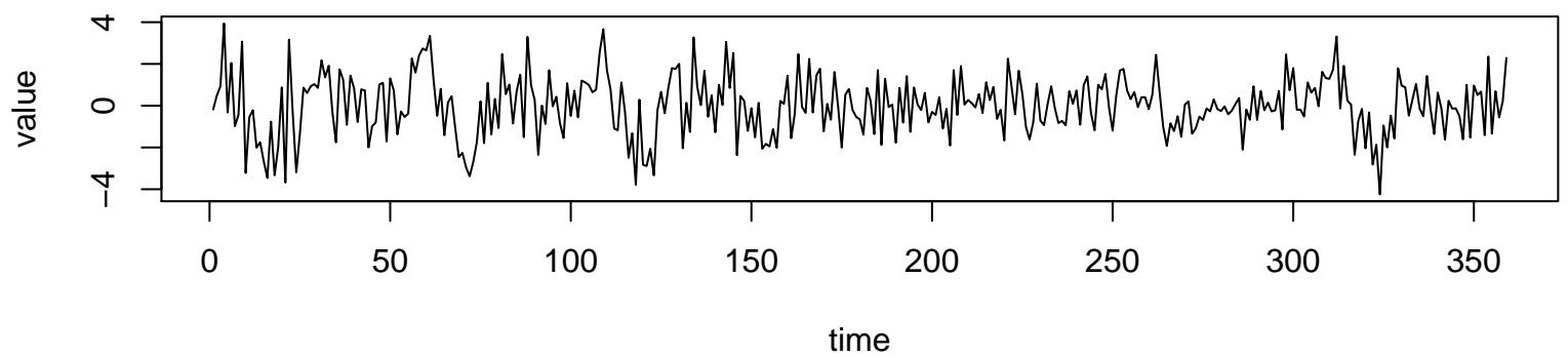
Working Time Series ( \lambda=0.5 , d=1 , D=1 )
