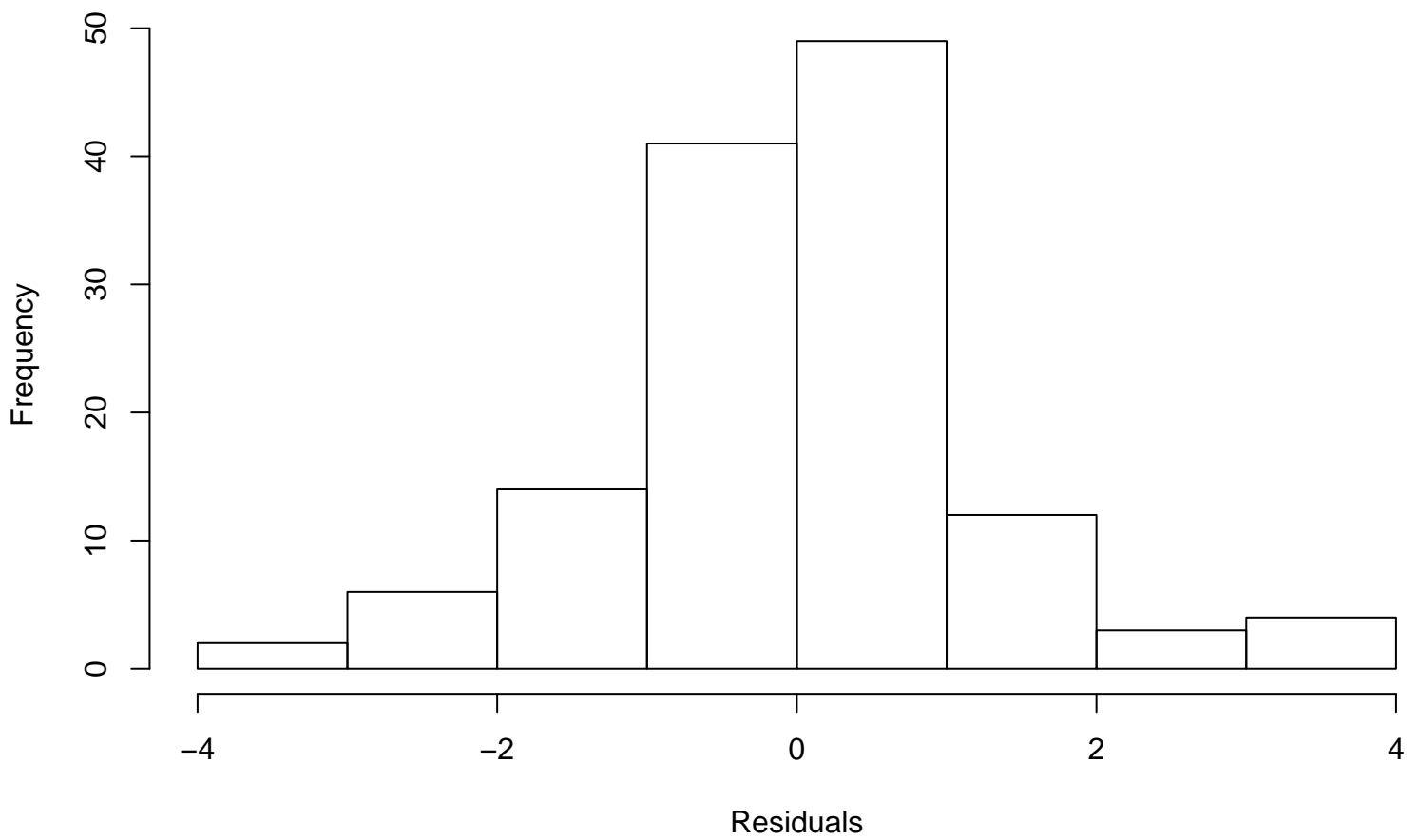
Residual Histogram
