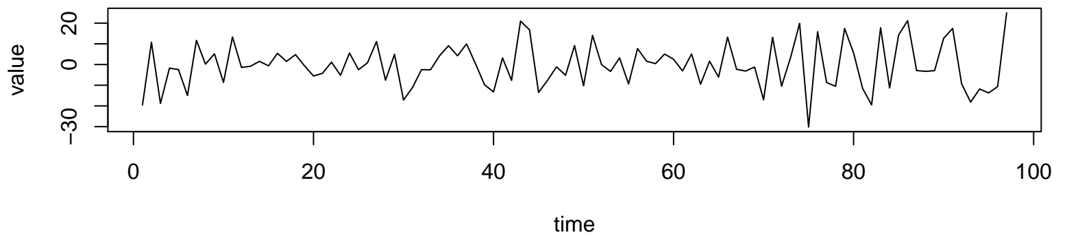
Working Time Series ( \lambda=1 , d=2 , D=1 )
