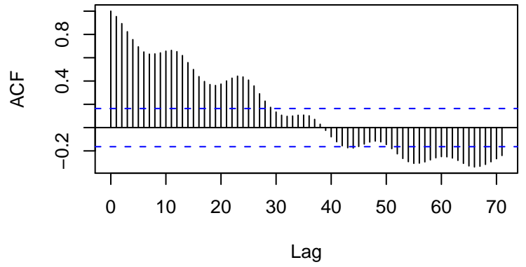
Standardized Residuals
