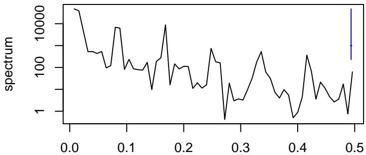
frequency bandwidth = 0.00231
