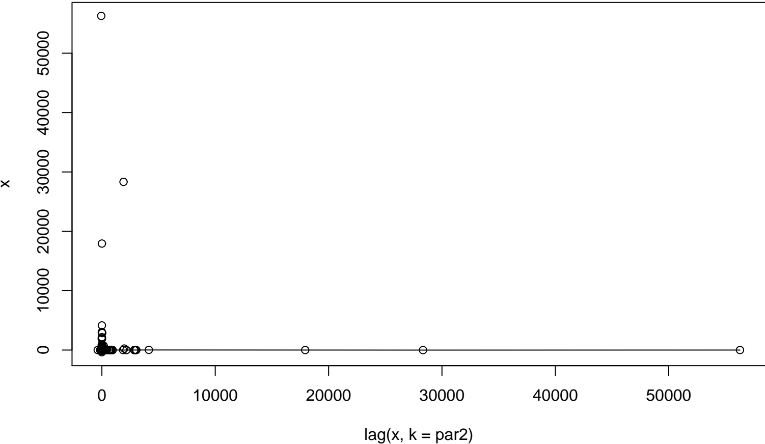
Lag plot (k=20), and lowess
