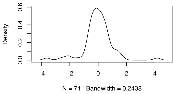
Residual Kernel Density
