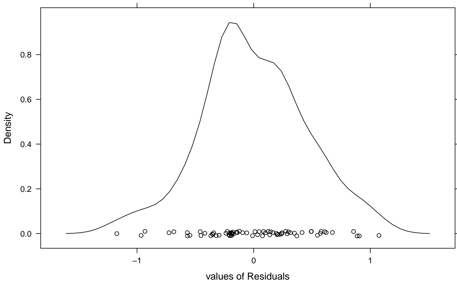
Residual Density Plot
