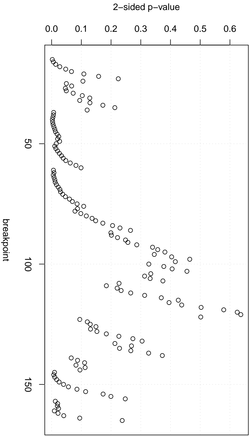
Goldfeld-Quandt test
