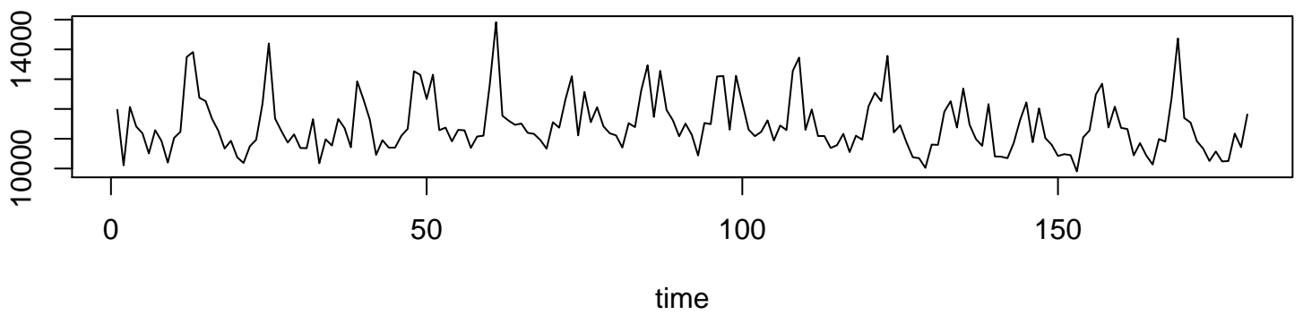
Working Time Series ( \lambda=1, d=0, D=0 )
