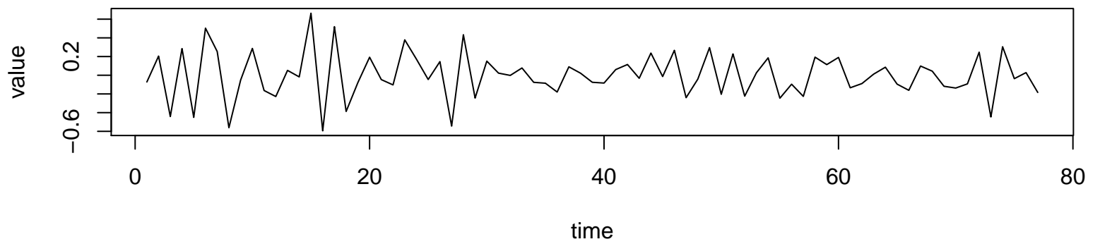
Working Time Series ( \lambda=1, d=1, D=1 )
