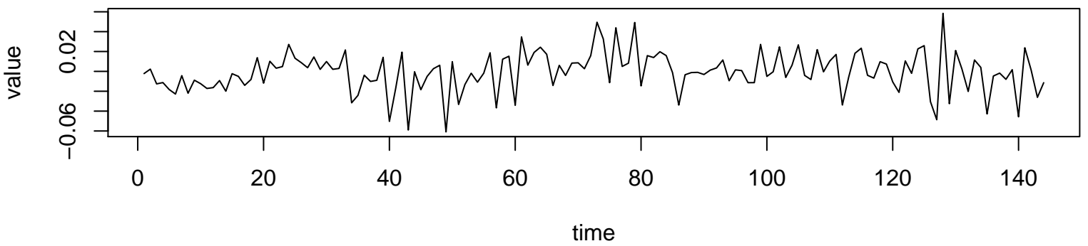
Working Time Series ( \lambda=-0.2 , d=0 , D=1 )
