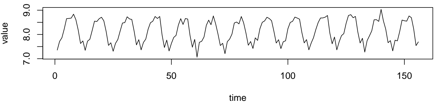
Working Time Series (lambda=0, d=0, D=0)
