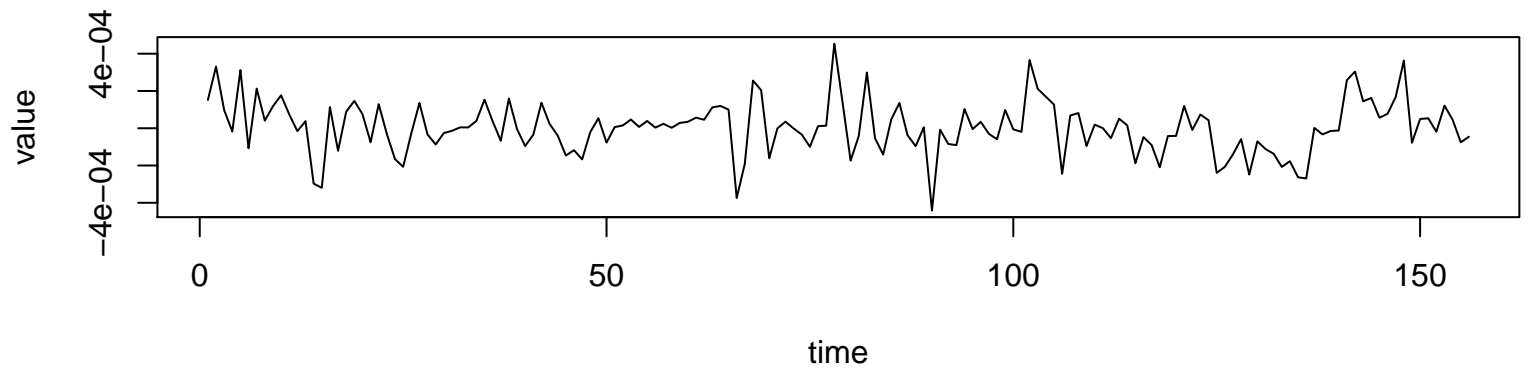
Working Time Series ( \lambda=-0.8 , d=0 , D=1 )
