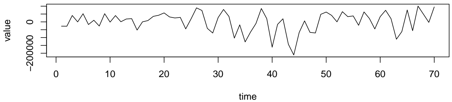
Working Time Series (lambda=2, d=1, D=0)
