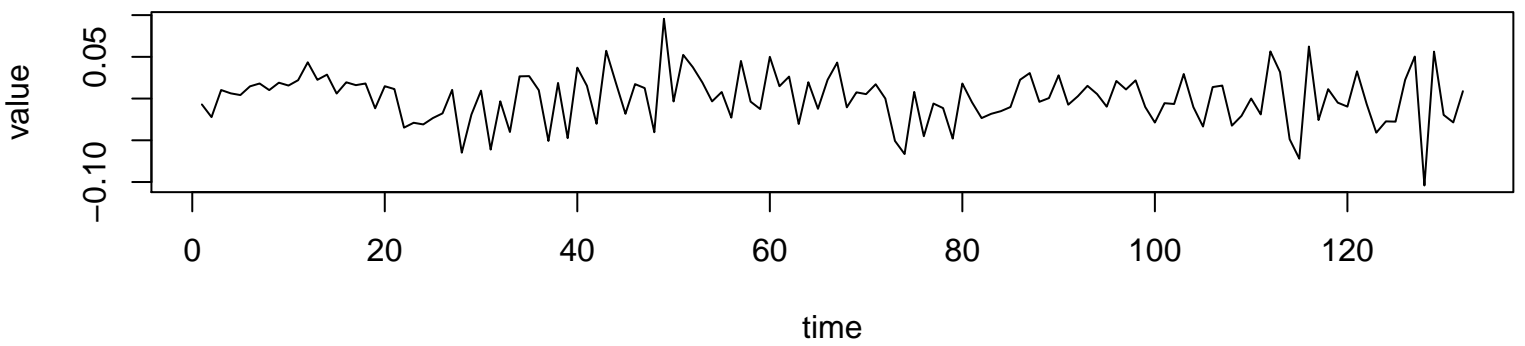
Working Time Series ( \lambda=-0.2 , d=0 , D=2 )
