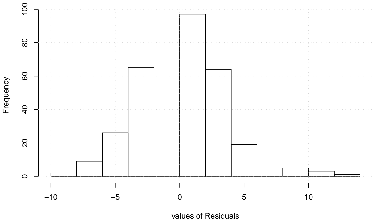
Residual Histogram
